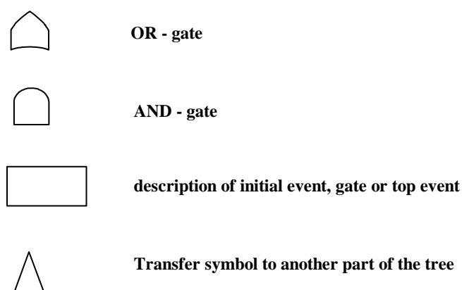
Figure I.2 Fault tree symbols
