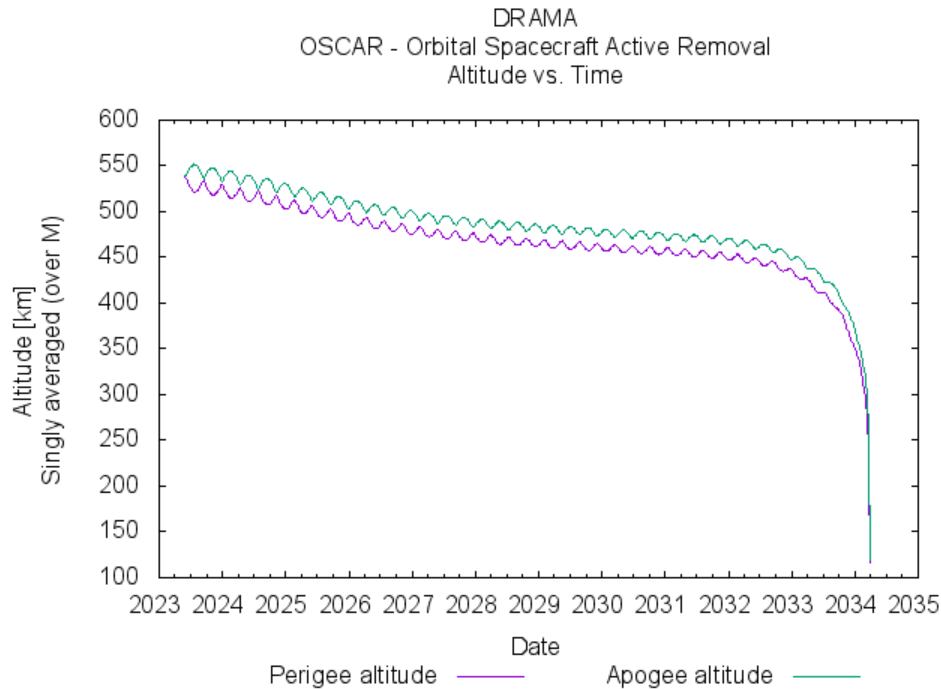
Figure 92: Satellite altitude over time – worst case with deployment failure of both SAA
