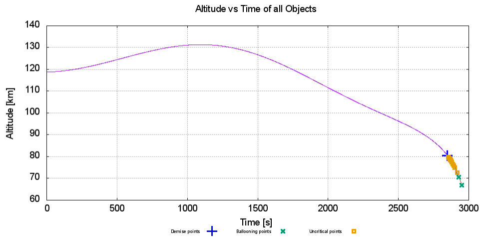
Figure 14. Altitude vs time for satellite components
