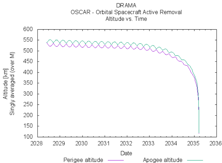
Figure 1: Satellite altitude over time – nominal cross section after end of 5 year mission
