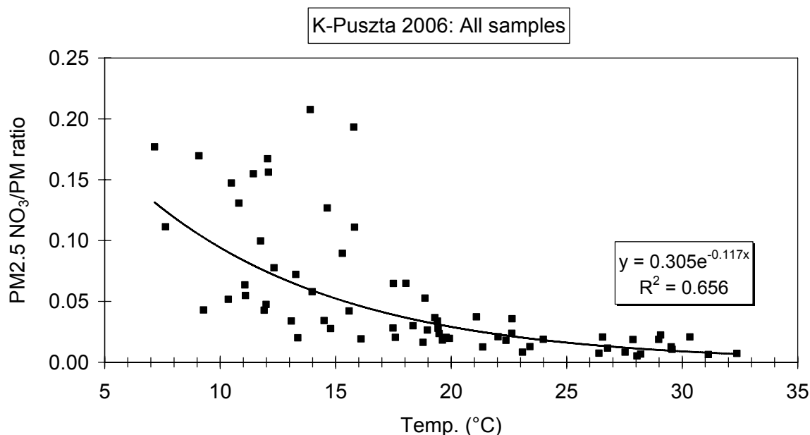
Figure 9. Relationship between the \text{NO}_3/\text{PM} ratio in \text{PM}_{2.5} and the air temperature for the filter samples of the 2006 summer campaign at K-pusztta.
