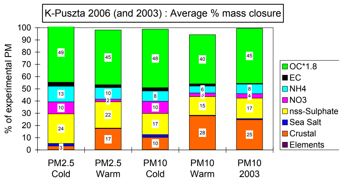
Figure 13. Percentage contributions of the various components to the average gravimetric PM for the 2006 summer campaign at K-pusztta, and this separately for the PM 2.5 and PM 10 aerosol and for the cold and warm periods. The data for the PM 10 aerosol during the 2003 summer campaign at the same site are also shown.
