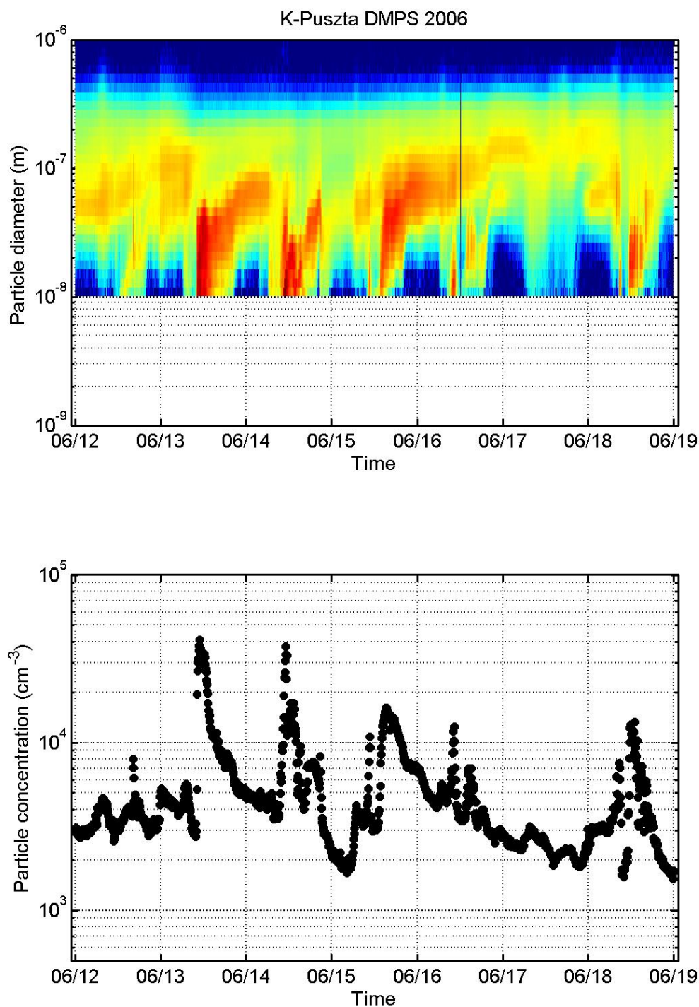
Figure 10. Particle size distribution and total concentration measured at the K-pusztá site with the DMPS during the week from 12 to 19 June 2006. The vertical dashed lines are at 00:00 h.
