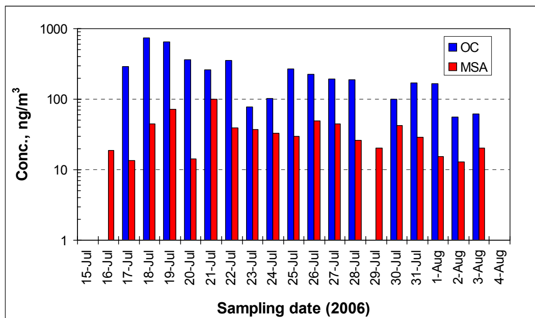
Figure 33. Time series for the OC and MSA concentrations in the fine ( <1.3 \mu\text{m} ) size fraction of the aerosol samples collected during the NH cruise.
