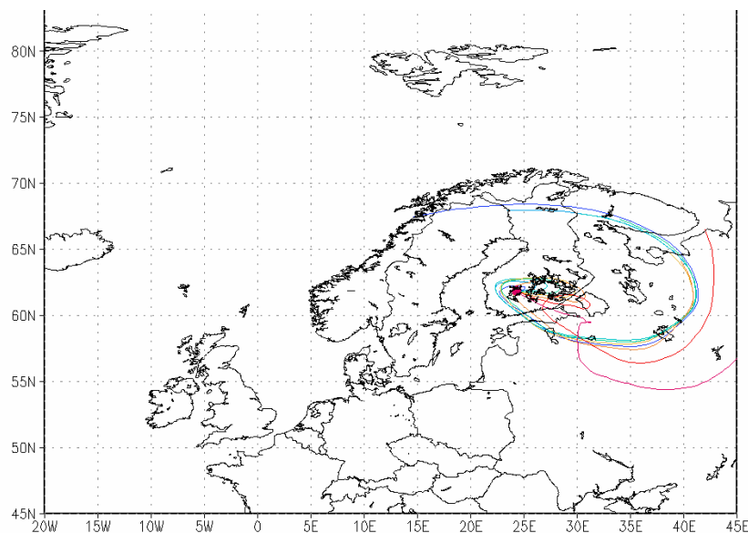
Figure 20. Five-day, 3-dimensional air mass back trajectories, calculated with HYSPLIT [Lupu and Maenhaut, 2002] for every 6 hours and for an arrival level of 100 m above ground at SMEAR II on 11 and 12 August 2007. The trajectories are colour-coded from dark blue to dark red, with the dark blue one for arrival on 11 August 0:00 UTC and the dark red one for 12 August 18:00 UTC.
