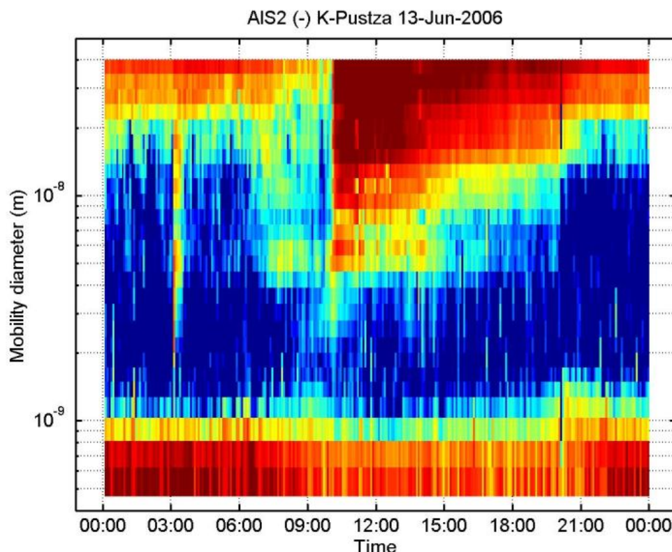
Figure 11. AIS air negative ion size distribution at the K-pusztá site during the day of 13 June 2006.
