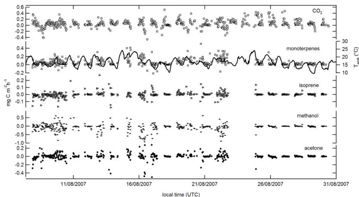
Figure 18. Time series of fluxes calculated with the profile-gradient technique for (from top to bottom): \text{CO}_2 , temperature and monoterpenes, isoprene, methanol, and acetone.
