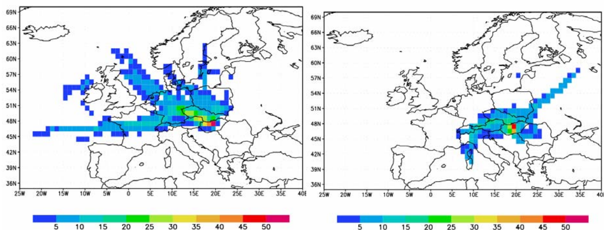
Figure 2. Air mass origin for the cold (left) and warm (right) periods of the 2006 summer campaign at K-pusztza. The plots show the number of trajectory crossings per grid cell (2.5° x 2.5° grid) in colour code for each of the two periods (only numbers of crossings of 4 and higher are depicted). The trajectories used were 5-day 3-dimensional back trajectories, calculated for every 6 hours and for an arrival level of 100 m above ground (The results for an arrival level of 300 m above ground were fairly similar).
