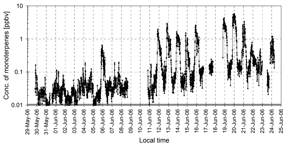
Figure 5. Time series of the atmospheric concentration of monoterpenes ( m/z 137) at K-pusztá for the period from 29 May to 25 June 2006. The vertical dashed lines are at 00:00 h.
