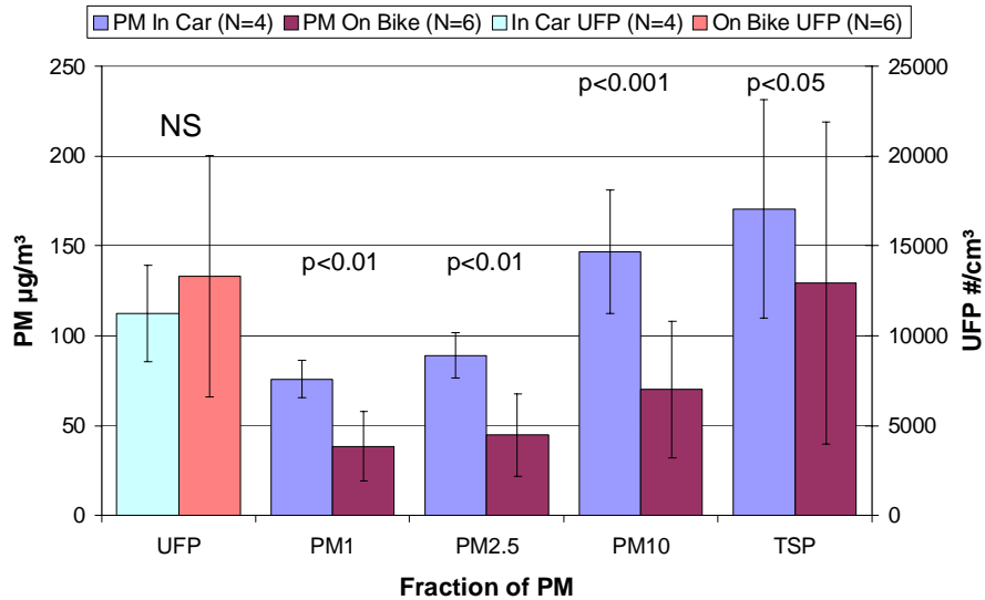
Figure 14: UFP numbers (right axis) and concentrations of PM fractions (left axis) for cyclists and car drivers respectively. Average concentrations ( 2 \times Standard deviation, paired t-test). PM concentrations are higher in the car than on the bicycle. UFP numbers are not significantly different.
