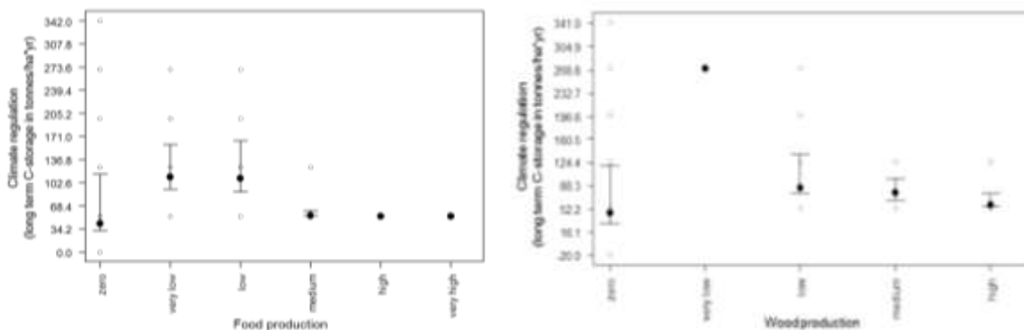
Figure 14 - Second level trade-off between food production and climate regulation (left) and wood production and climate regulation (right) in the Nete basin case study. Grey dots represent feasibility values occurring within the study area (one for each pixel, of which many superposed on each other by model outcomes). Black dots represent mean values, error bars represent asymmetric standard deviations distributed according to relative position of the mean.
